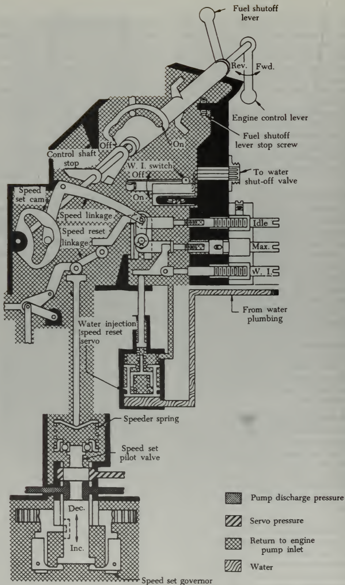
FIGURE 3-53. Water injection re-set system.
